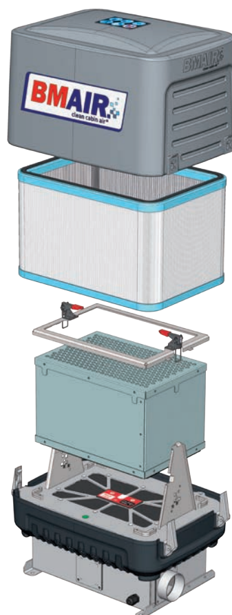
MAO-3 Cab Guard active carbon combination
